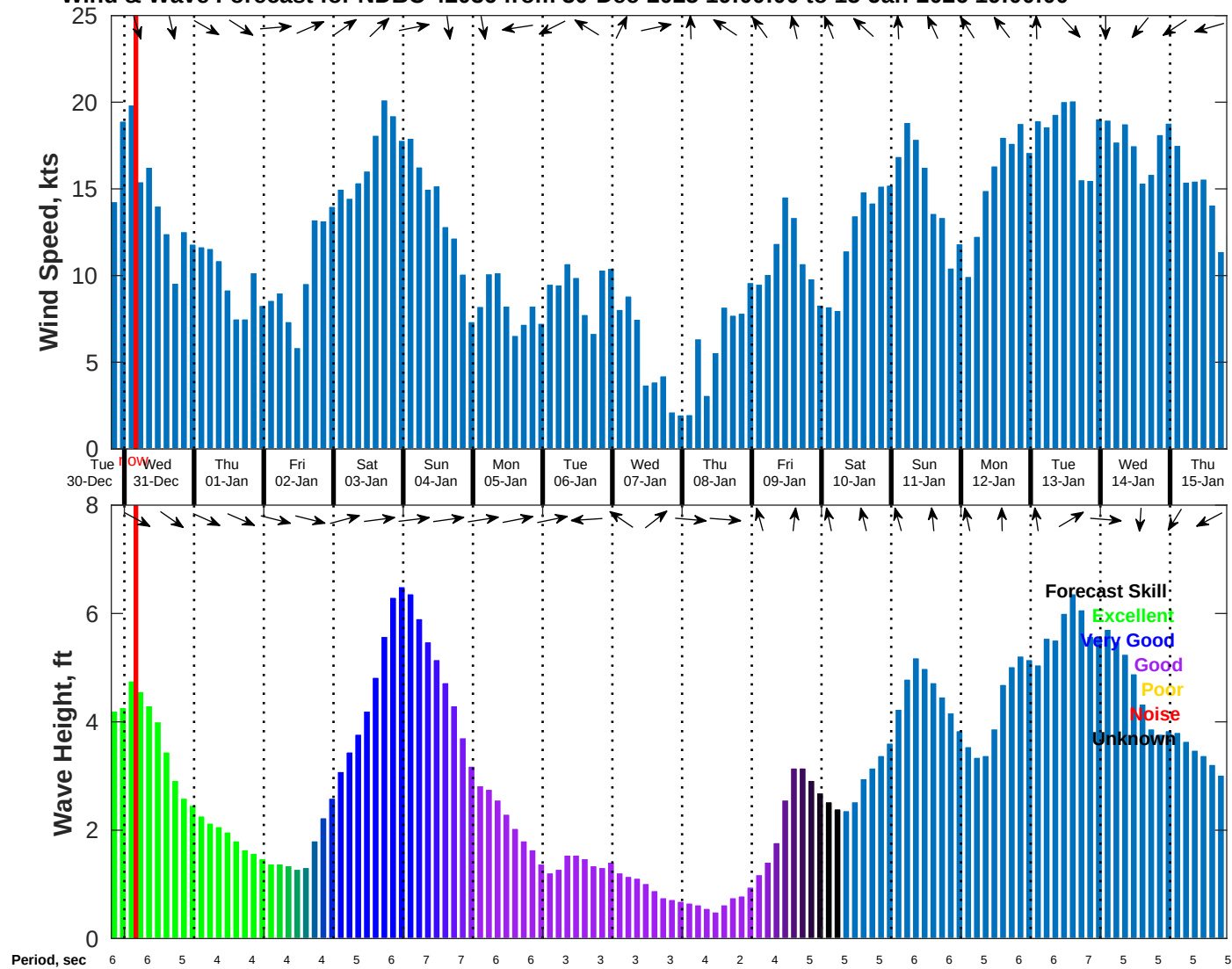
Wind & Wave Forecast for NDBC 42036 from 30-Dec-2025 19:00:00 to 15-Jan-2026 19:00:00
