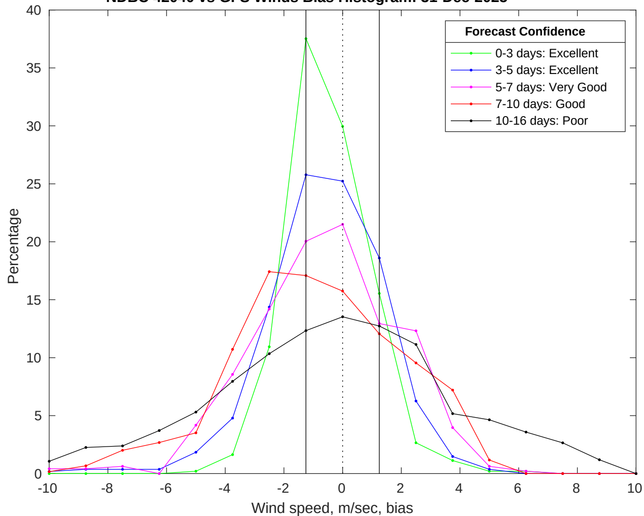
NDBC 42040 vs GFS Winds Bias Histogram: 31-Dec-2025
