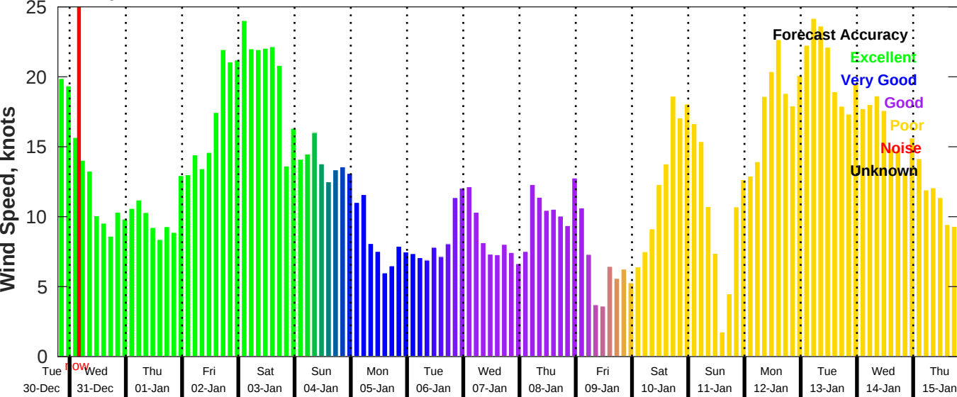
GFS Wind Speed Forecast for NDBC 42040 from 30-Dec-2025 19:00:00 to 15-Jan-2026 19:00:00
