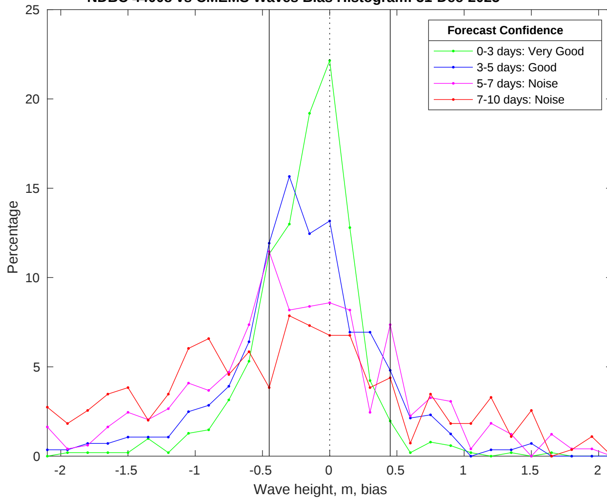
NDBC 44008 vs CMEMS Waves Bias Histogram: 31-Dec-2025
