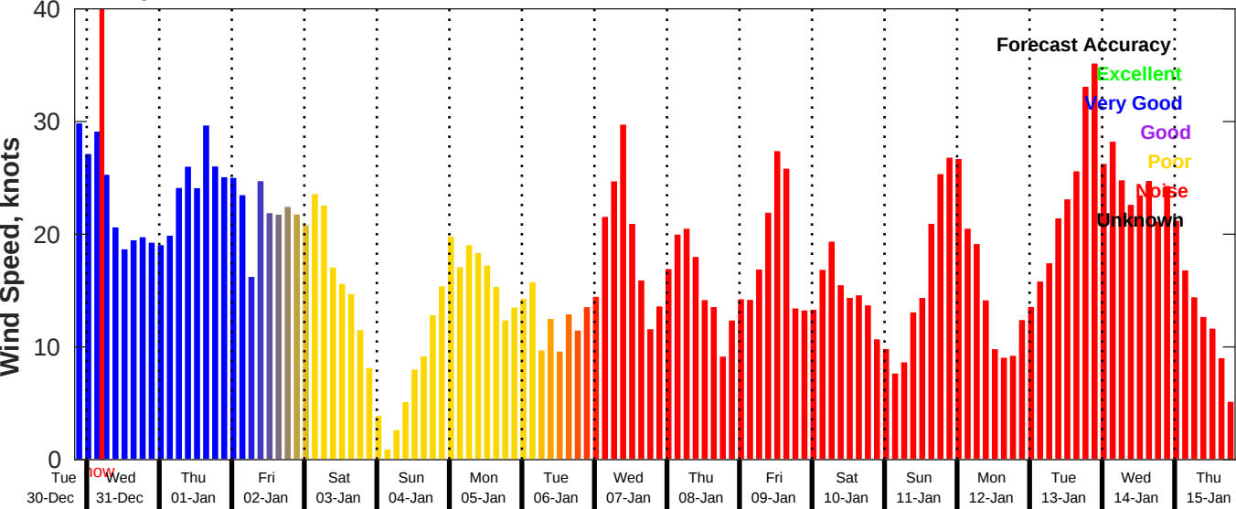
GFS Wind Speed Forecast for NDBC 44008 from 30-Dec-2025 20:00:00 to 15-Jan-2026 20:00:00
