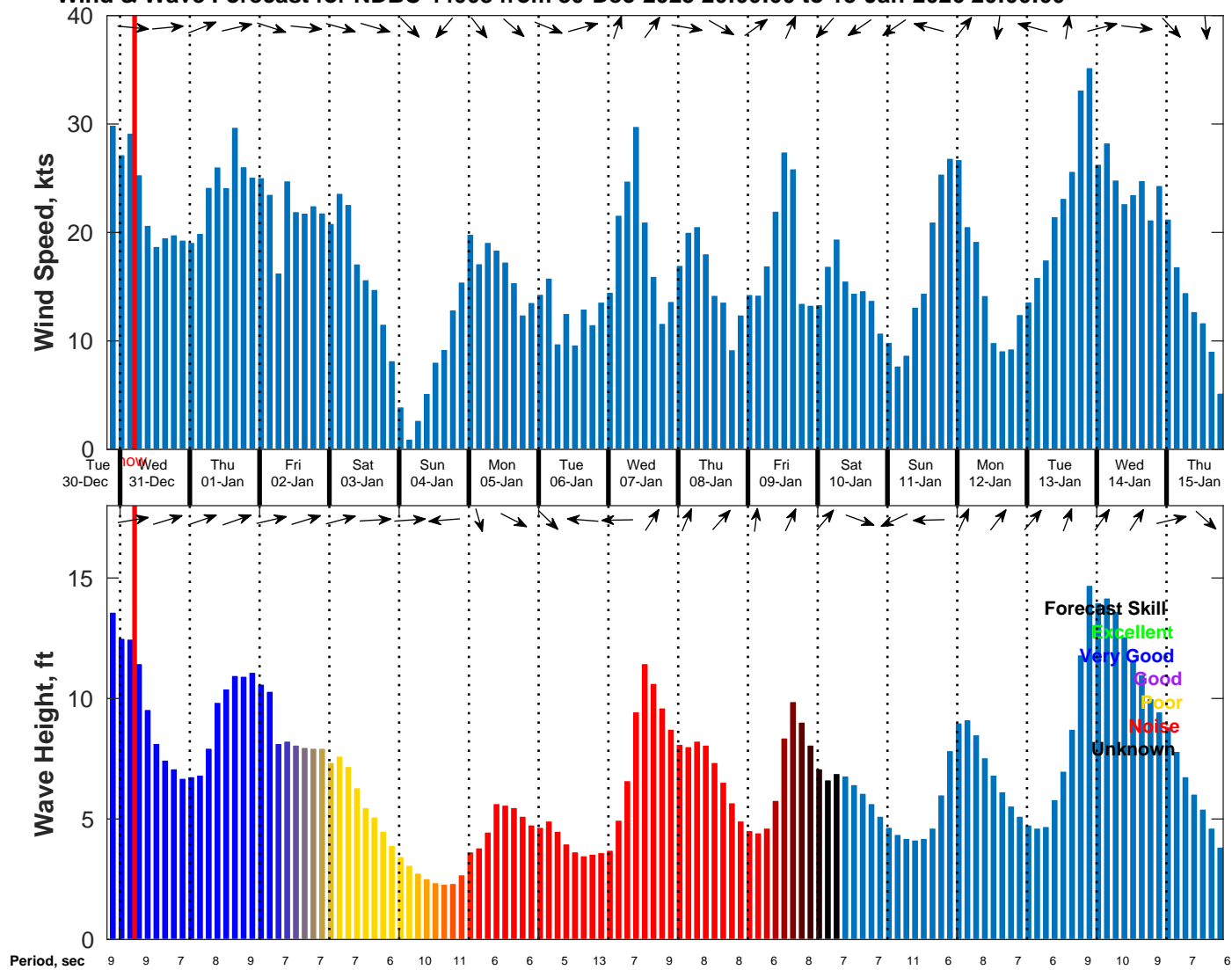
Wind & Wave Forecast for NDBC 44008 from 30-Dec-2025 20:00:00 to 15-Jan-2026 20:00:00
