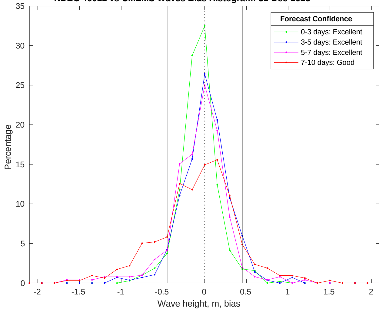
NDBC 46011 vs CMEMS Waves Bias Histogram: 31-Dec-2025
