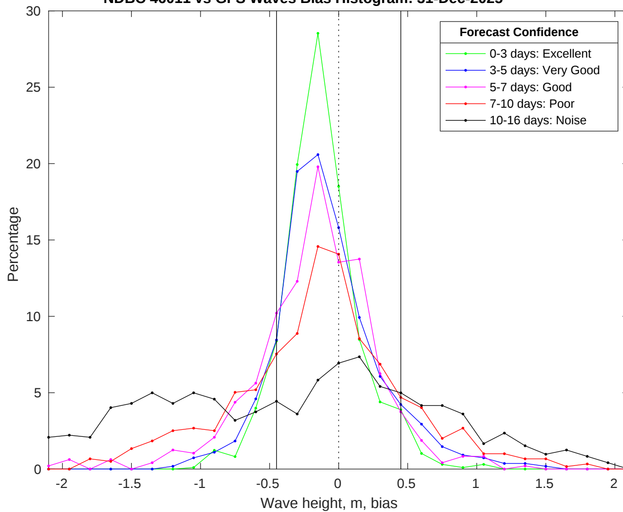
NDBC 46011 vs GFS Waves Bias Histogram: 31-Dec-2025
