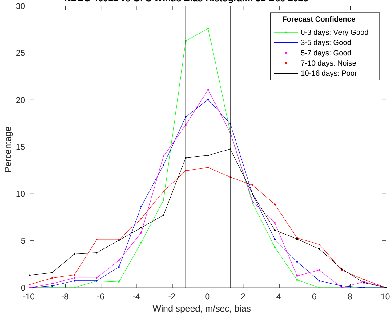
NDBC 46011 vs GFS Winds Bias Histogram: 31-Dec-2025
