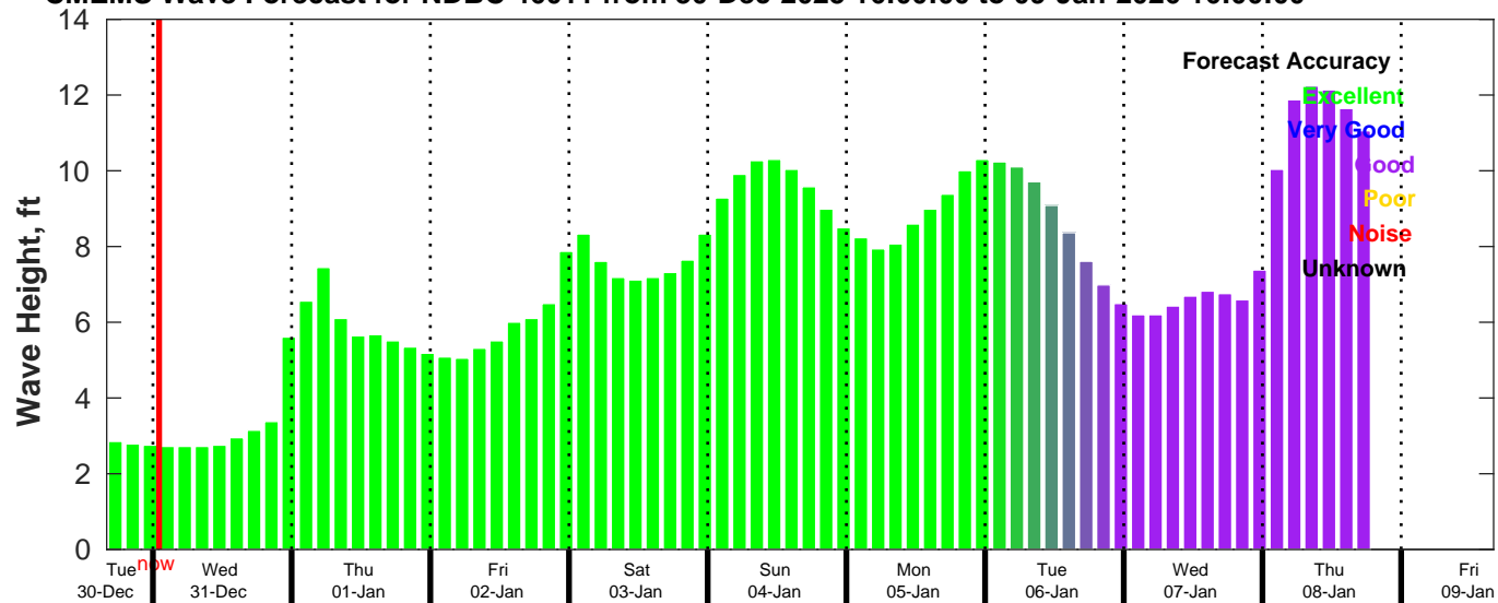
CMEMS Wave Forecast for NDBC 46011 from 30-Dec-2025 16:00:00 to 09-Jan-2026 16:00:00
