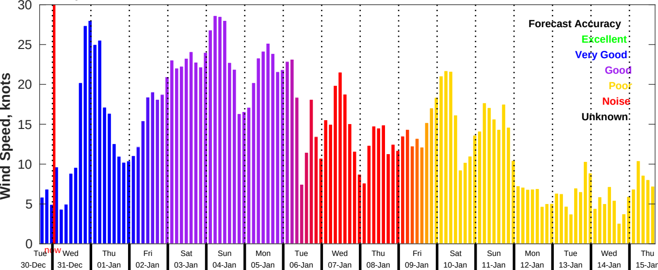
GFS Wind Speed Forecast for NDBC 46011 from 30-Dec-2025 16:00:00 to 15-Jan-2026 16:00:00
