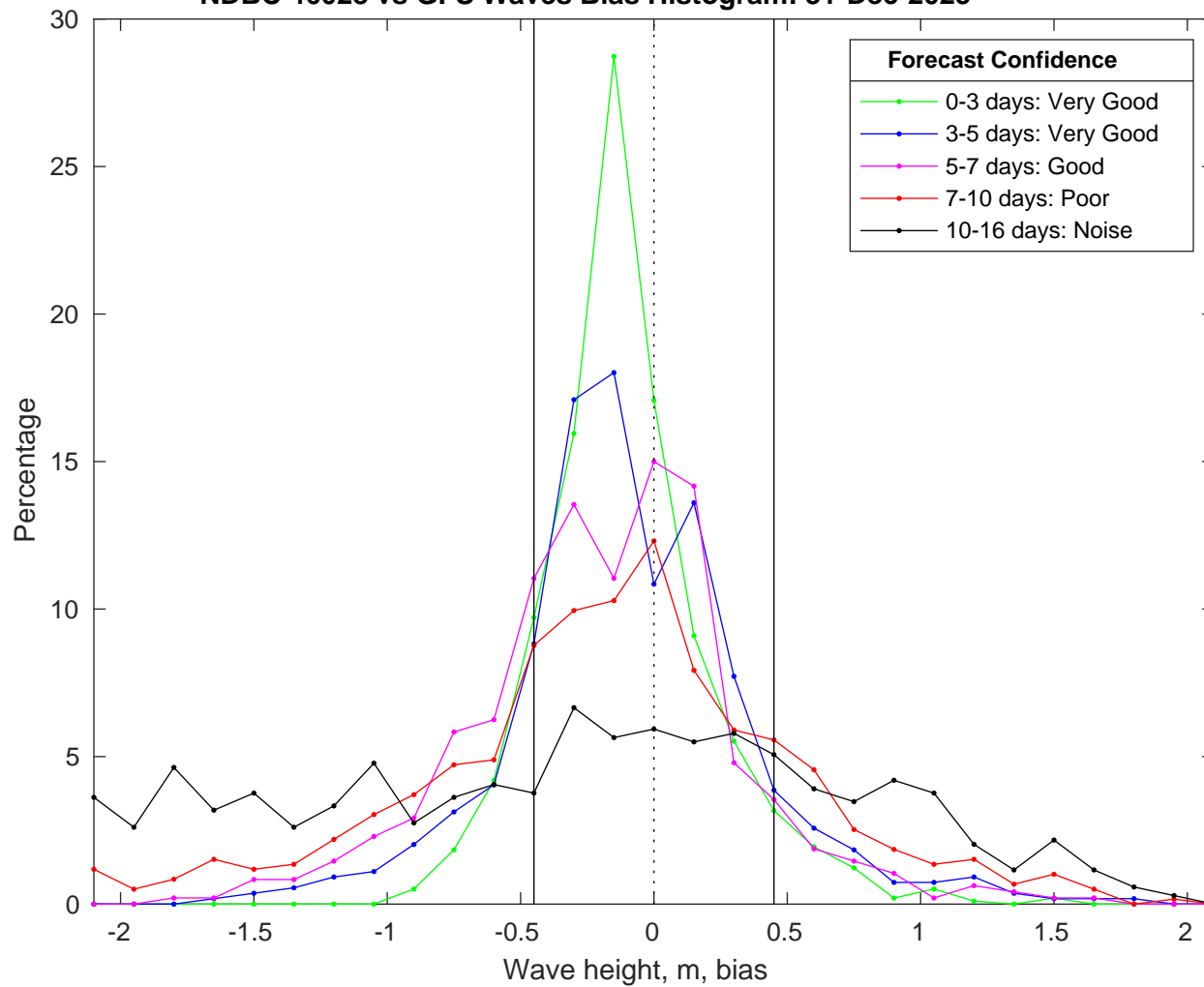
NDBC 46028 vs GFS Waves Bias Histogram: 31-Dec-2025
