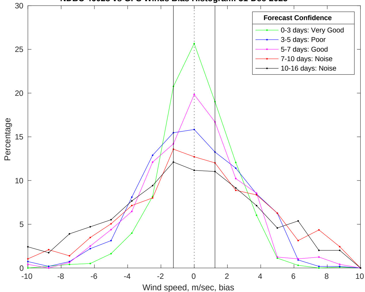
NDBC 46028 vs GFS Winds Bias Histogram: 31-Dec-2025
