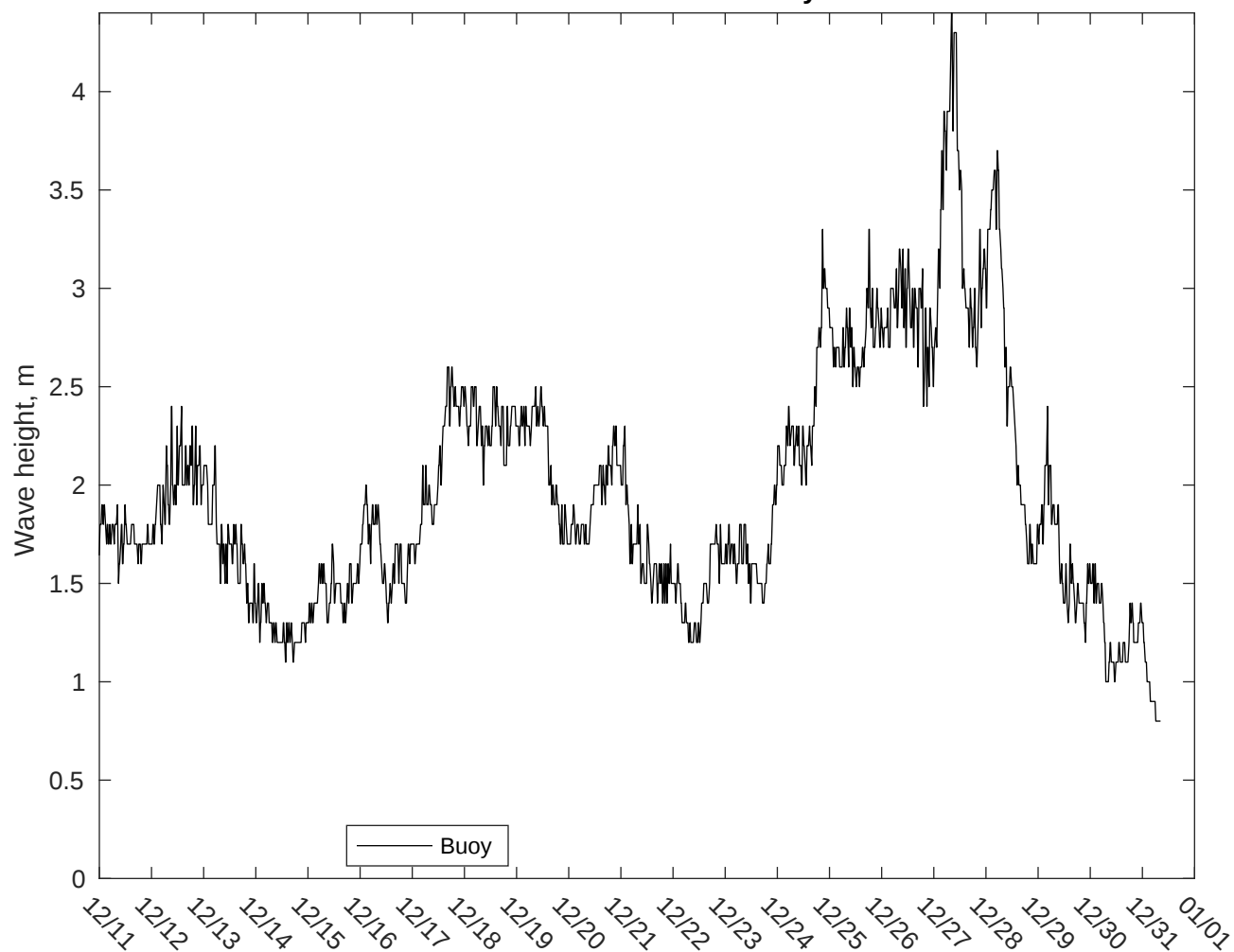
NDBC 46054 vs CMEMS Waves: 10 to 16 day forecast
