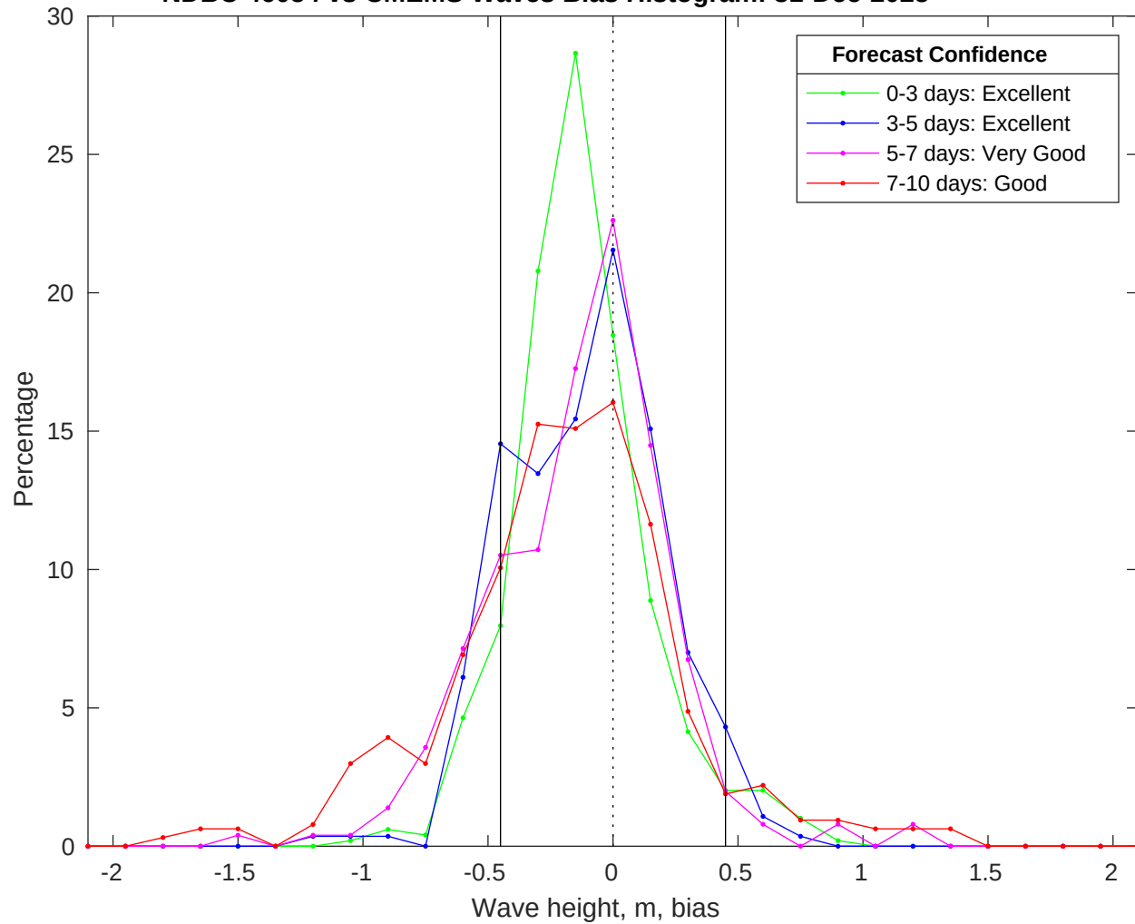
NDBC 46054 vs CMEMS Waves Bias Histogram: 31-Dec-2025
