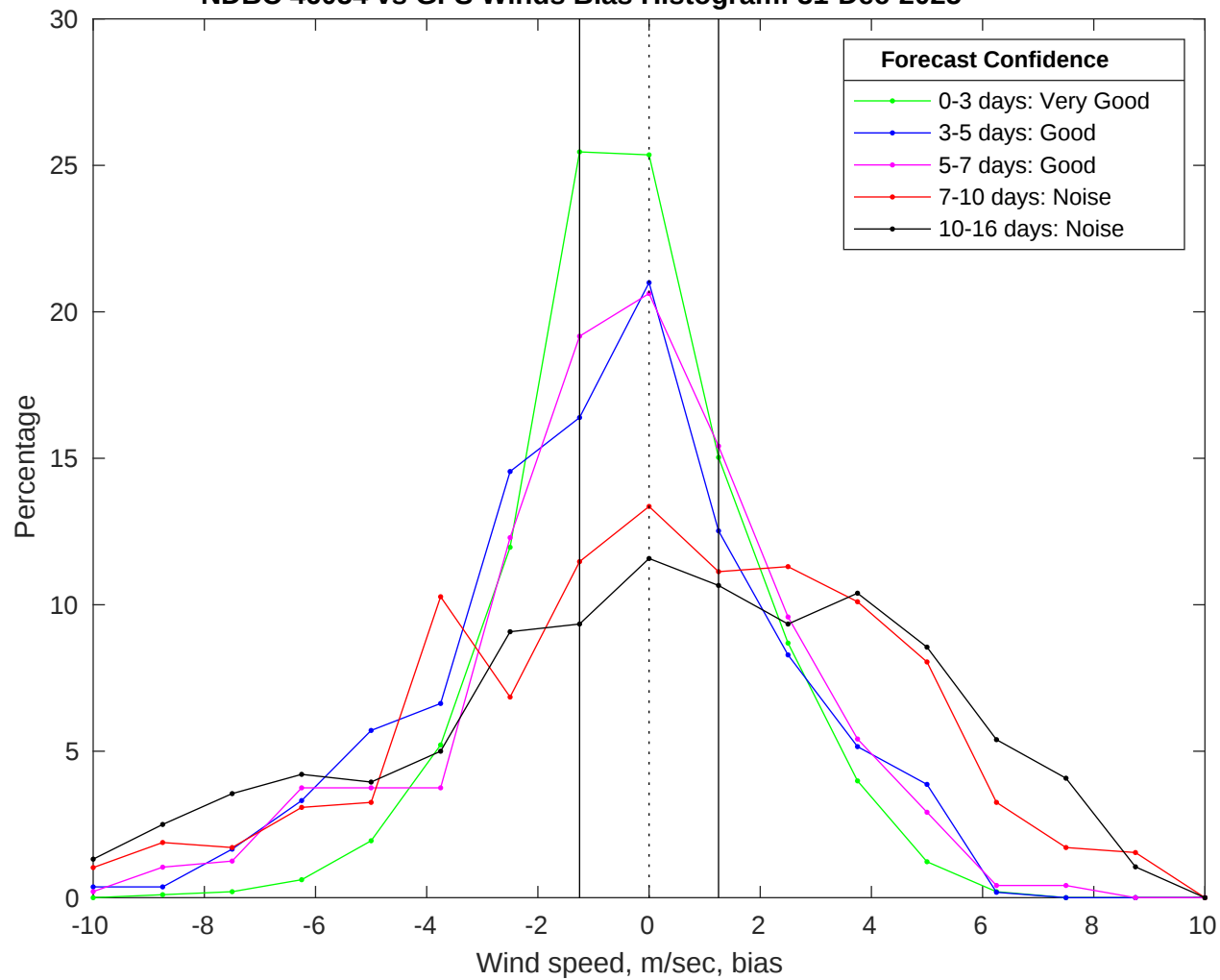
NDBC 46054 vs GFS Winds Bias Histogram: 31-Dec-2025
