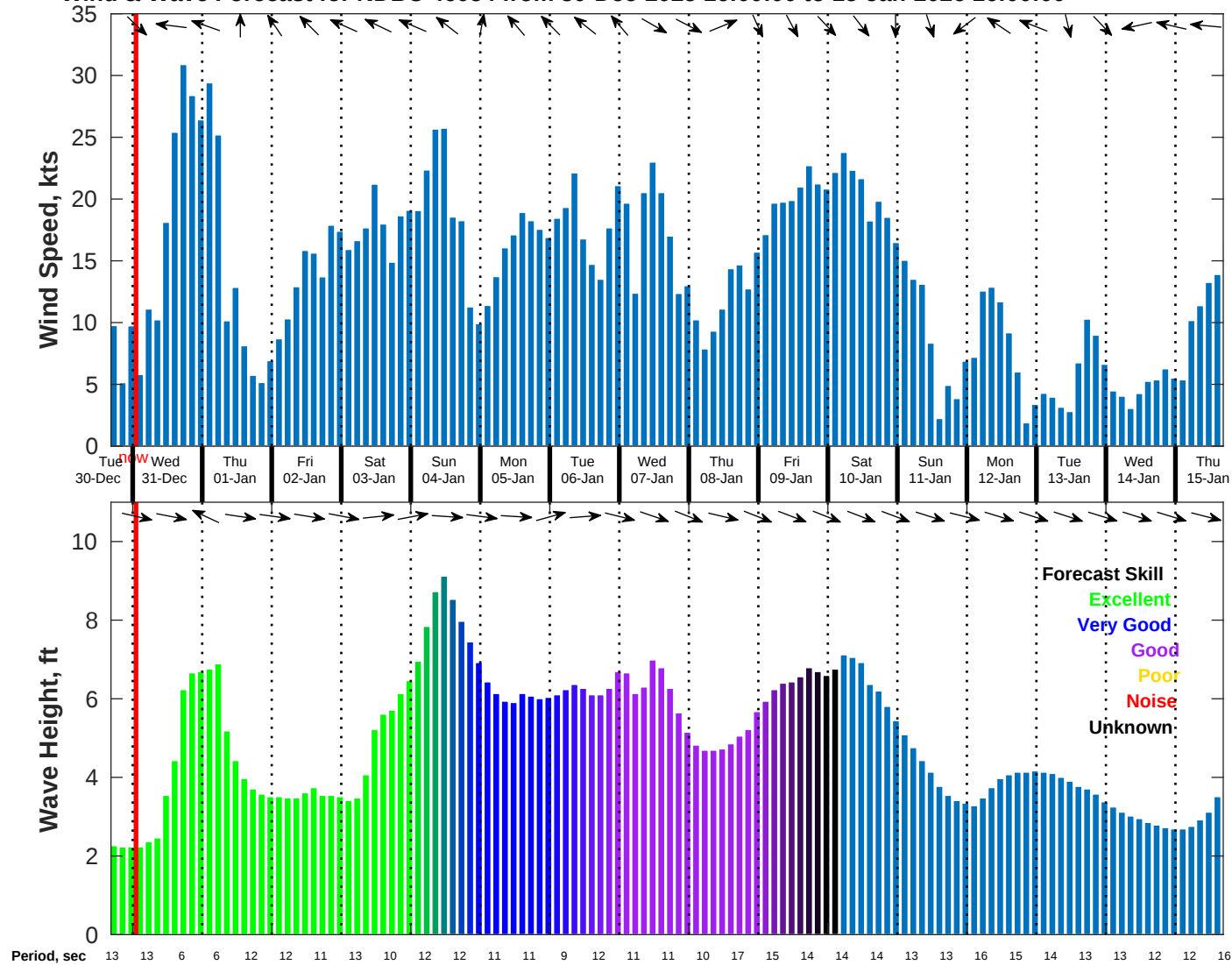
Wind & Wave Forecast for NDBC 46054 from 30-Dec-2025 16:00:00 to 15-Jan-2026 16:00:00
