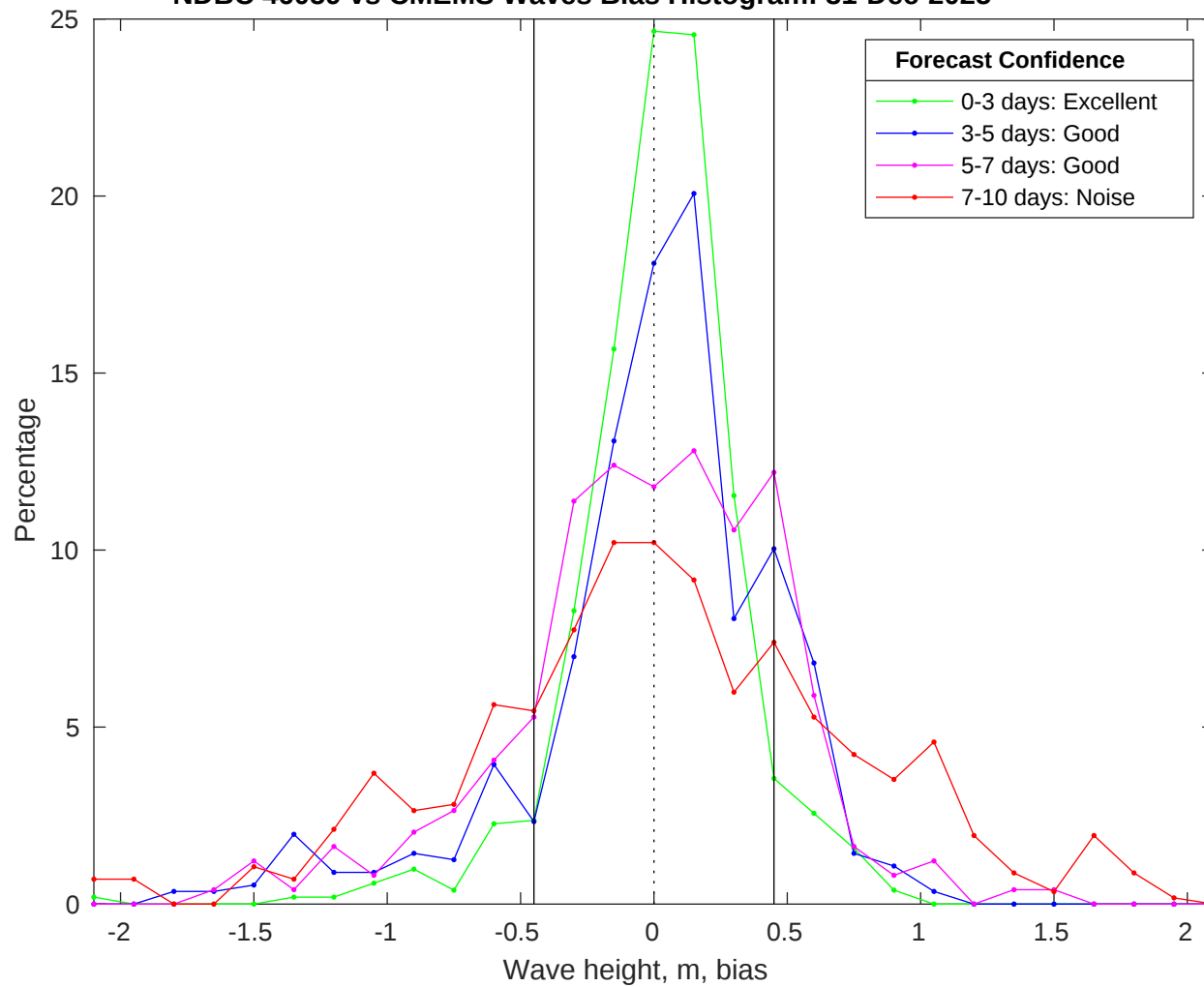
NDBC 46059 vs CMEMS Waves Bias Histogram: 31-Dec-2025
