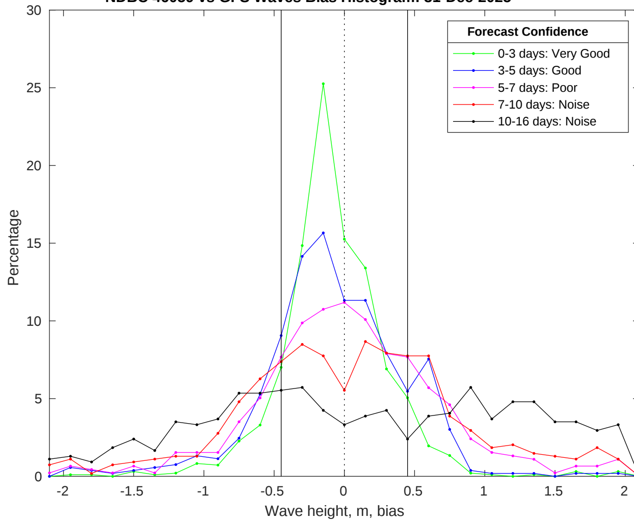
NDBC 46059 vs GFS Waves Bias Histogram: 31-Dec-2025
