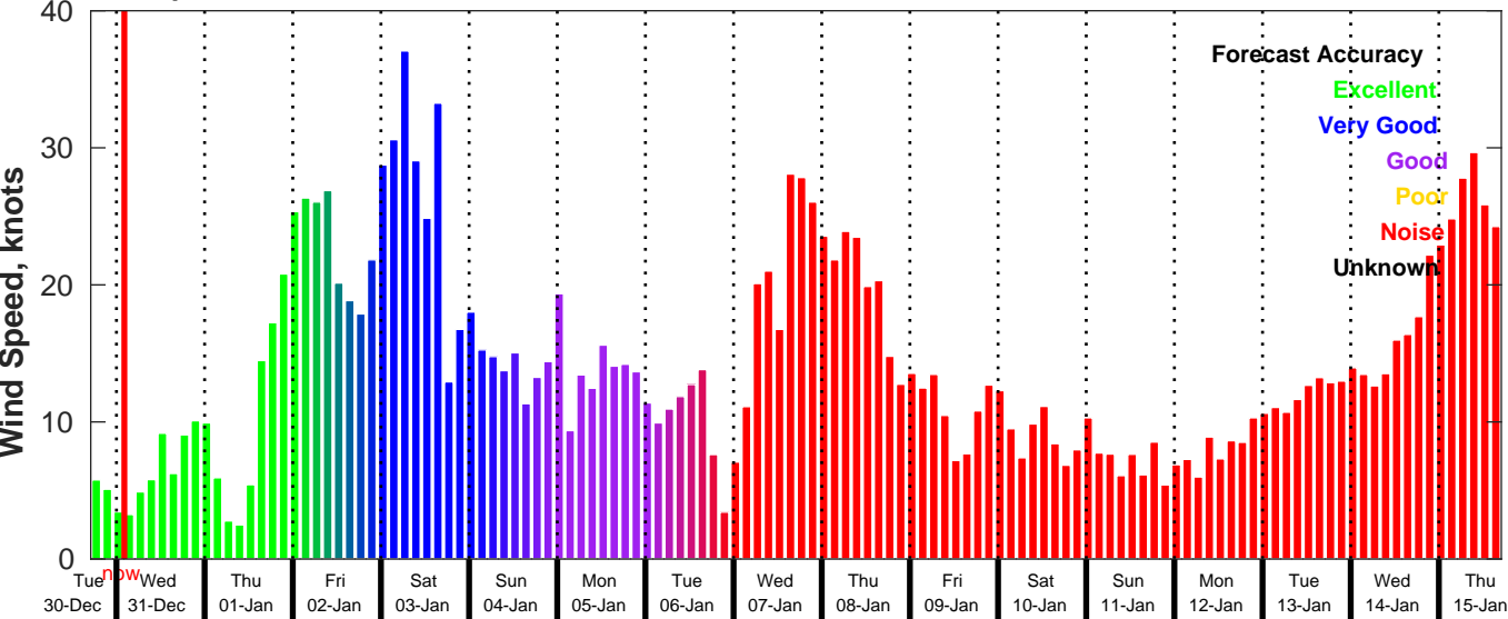
GFS Wind Speed Forecast for NDBC 46059 from 30-Dec-2025 17:00:00 to 15-Jan-2026 17:00:00
