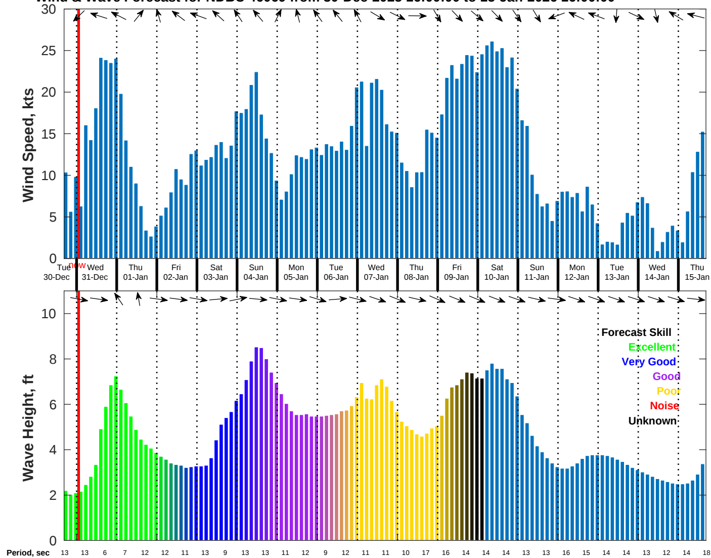
Wind & Wave Forecast for NDBC 46069 from 30-Dec-2025 16:00:00 to 15-Jan-2026 16:00:00
