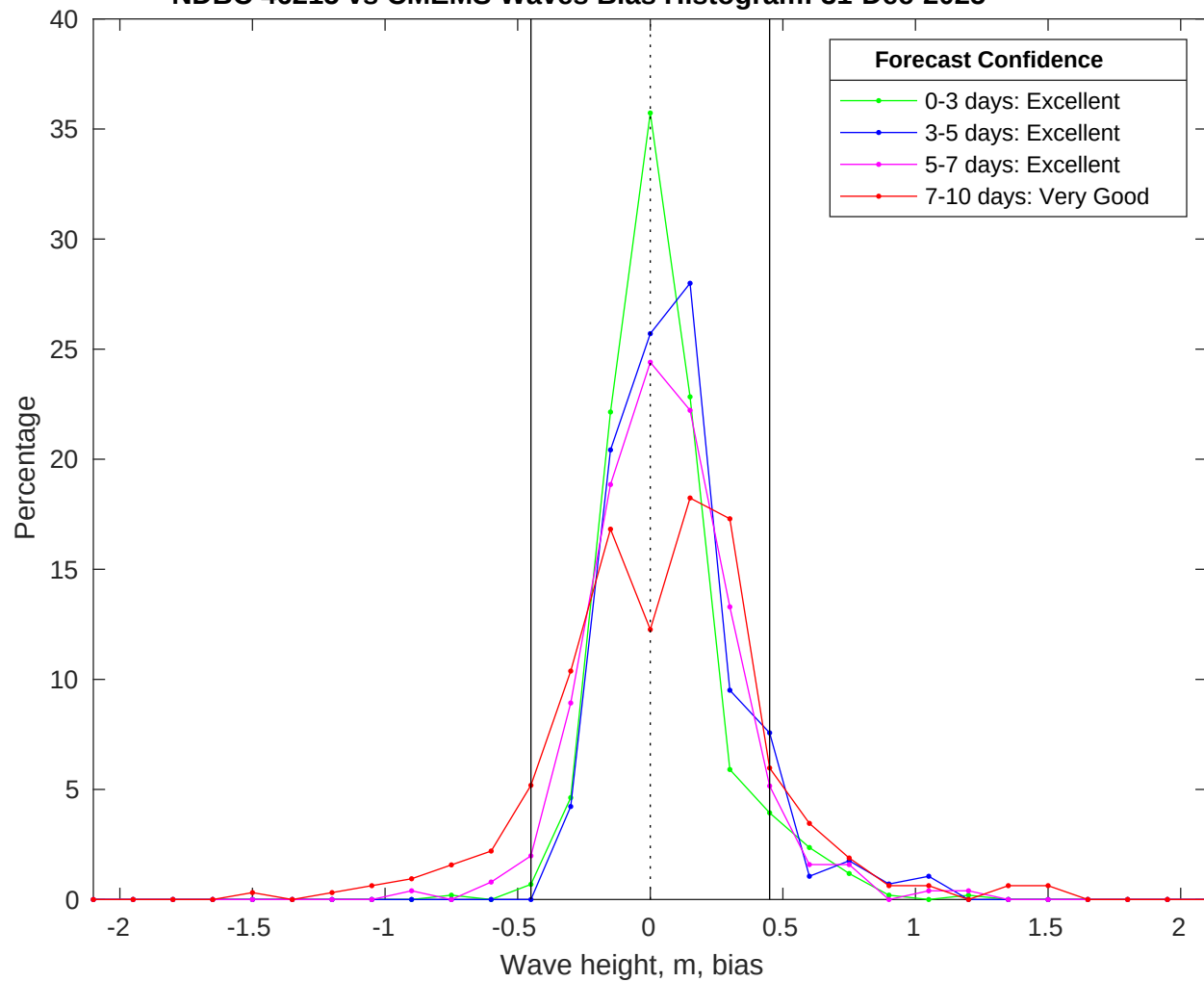
NDBC 46215 vs CMEMS Waves Bias Histogram: 31-Dec-2025
