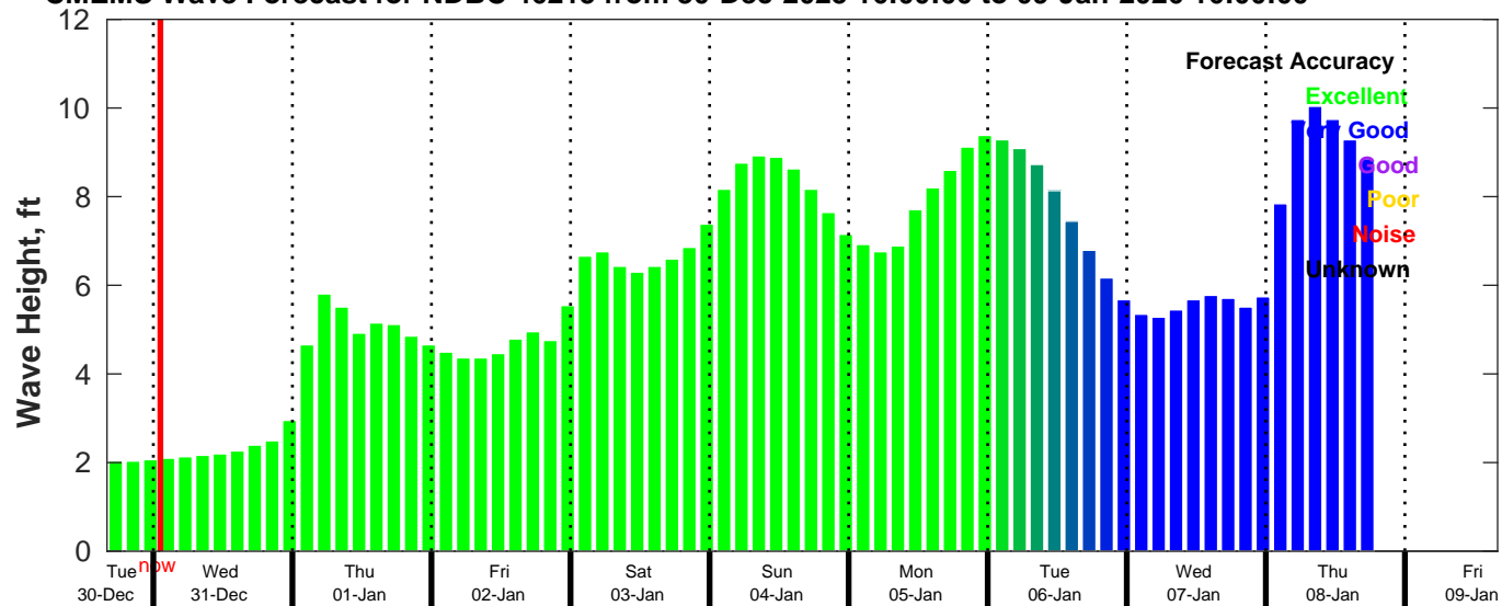
CMEMS Wave Forecast for NDBC 46215 from 30-Dec-2025 16:00:00 to 09-Jan-2026 16:00:00
