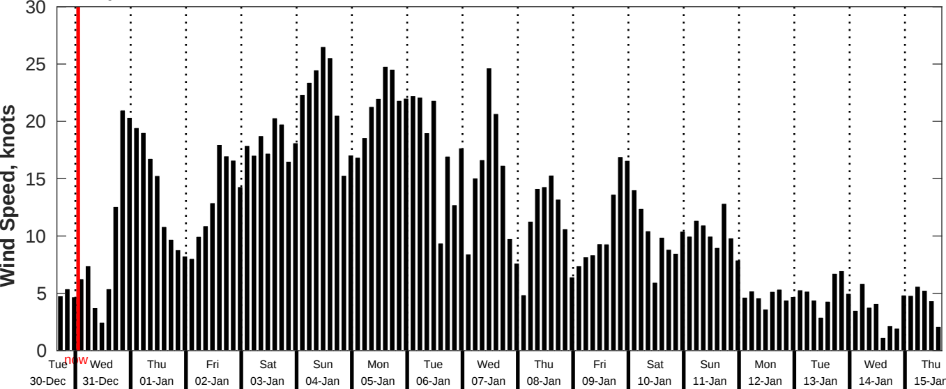
GFS Wind Speed Forecast for NDBC 46215 from 30-Dec-2025 16:00:00 to 15-Jan-2026 16:00:00
