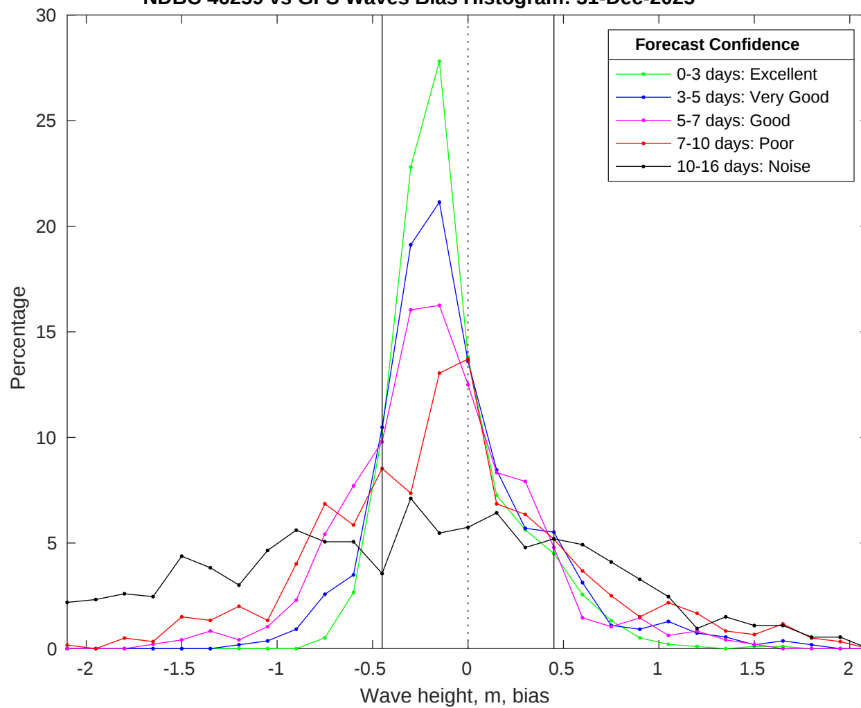
NDBC 46259 vs GFS Waves Bias Histogram: 31-Dec-2025
