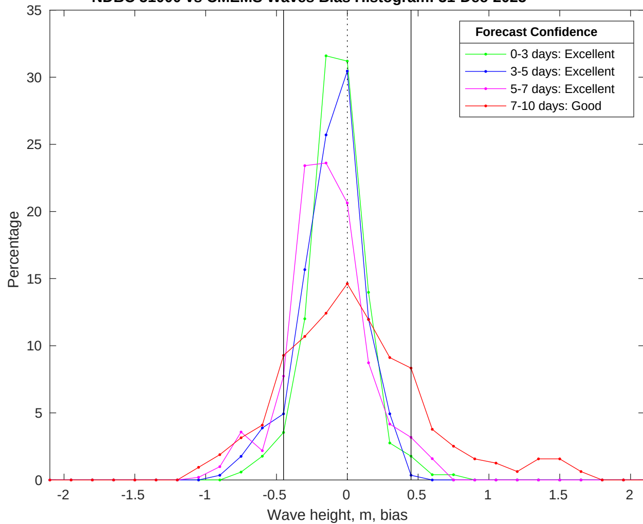
NDBC 51000 vs CMEMS Waves Bias Histogram: 31-Dec-2025
