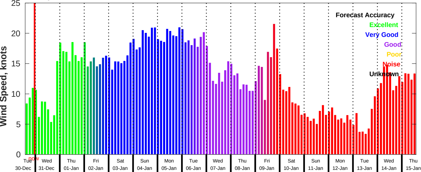
GFS Wind Speed Forecast for NDBC 51000 from 30-Dec-2025 14:00:00 to 15-Jan-2026 14:00:00
