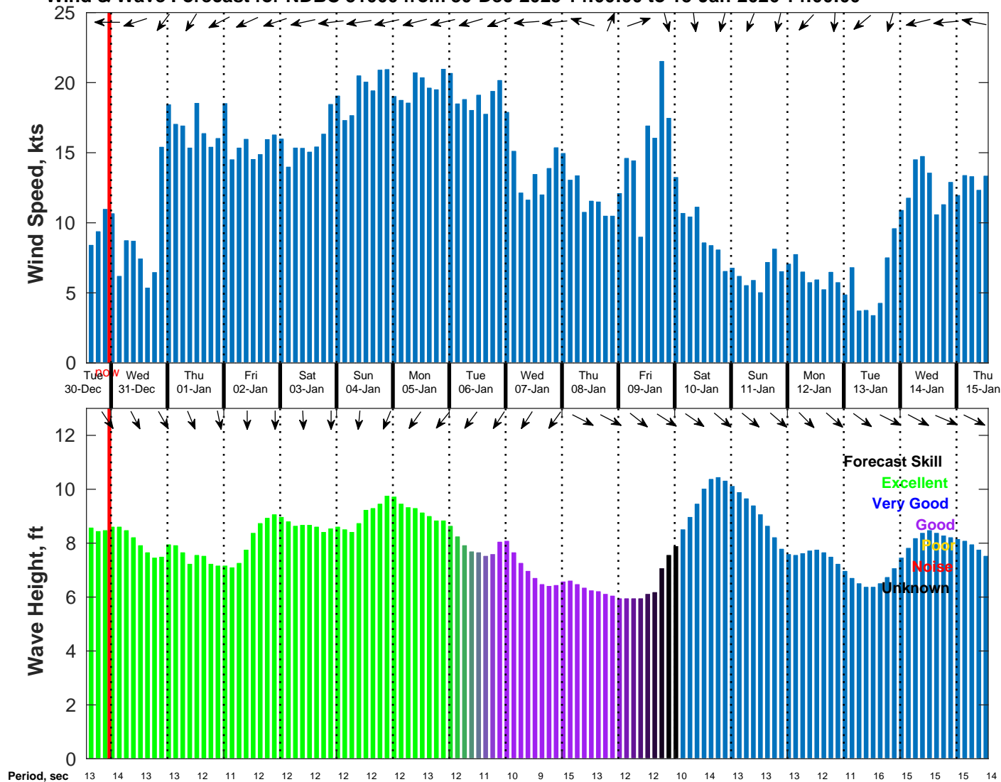
Wind & Wave Forecast for NDBC 51000 from 30-Dec-2025 14:00:00 to 15-Jan-2026 14:00:00
