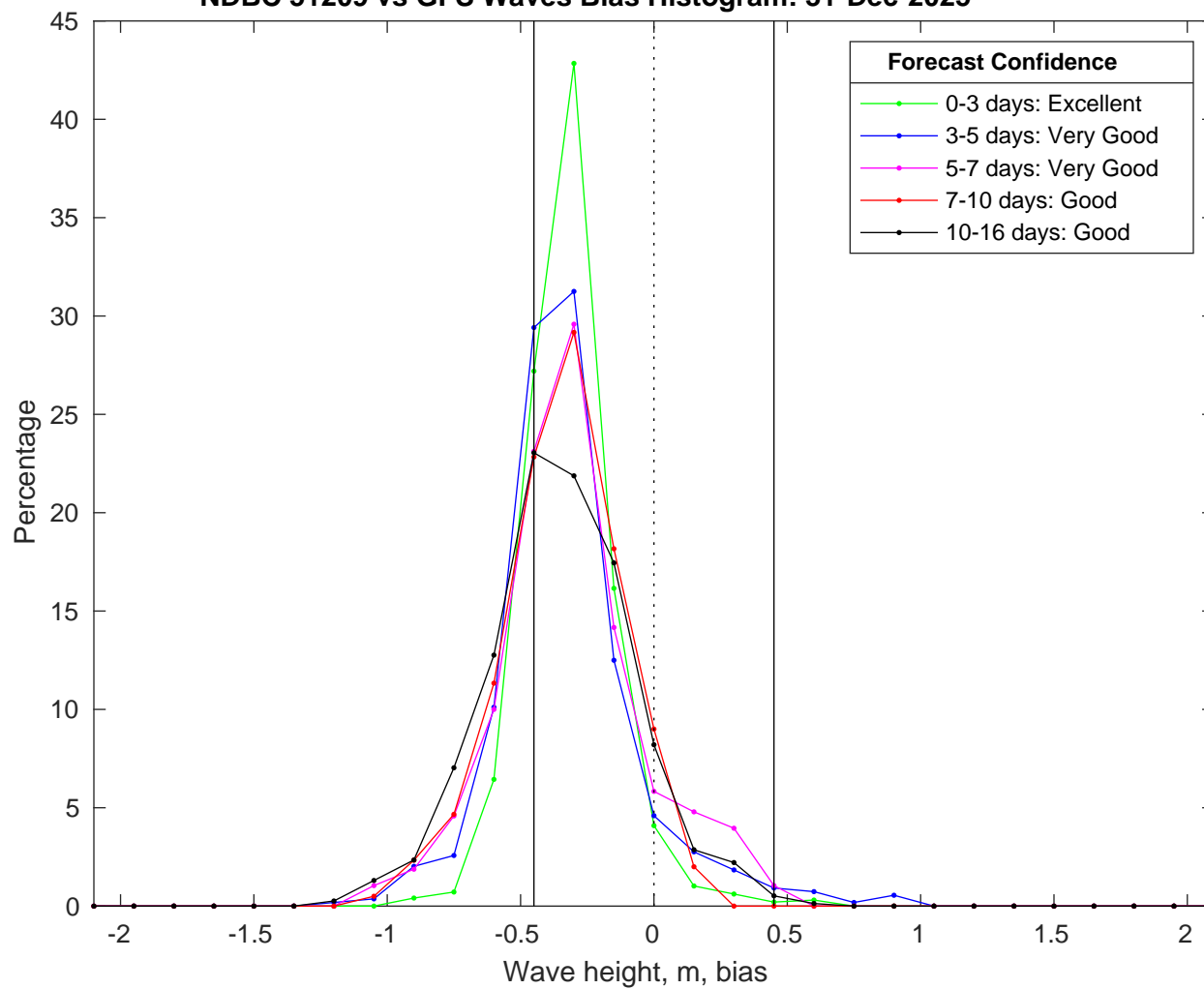
NDBC 51209 vs GFS Waves Bias Histogram: 31-Dec-2025
