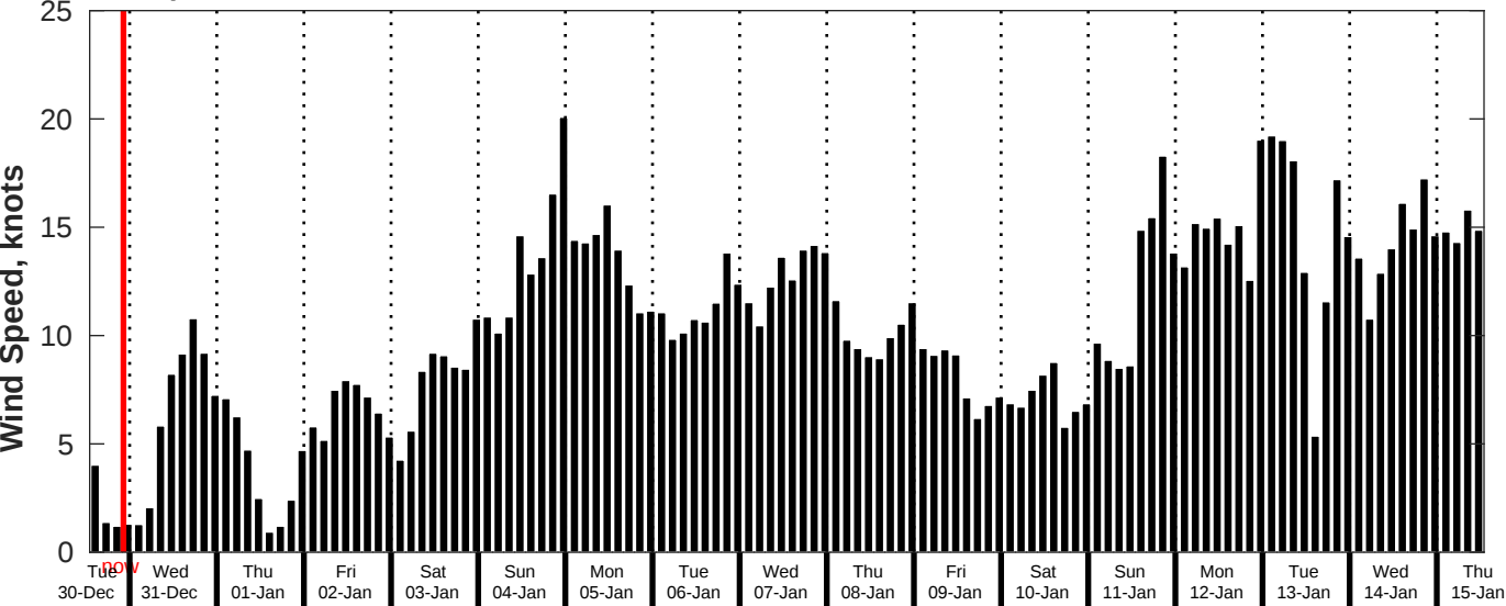
GFS Wind Speed Forecast for NDBC 51209 from 30-Dec-2025 13:00:00 to 15-Jan-2026 13:00:00
