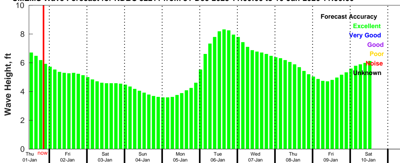
CMEMS Wave Forecast for NDBC 52211 from 31-Dec-2025 11:00:00 to 10-Jan-2026 11:00:00
