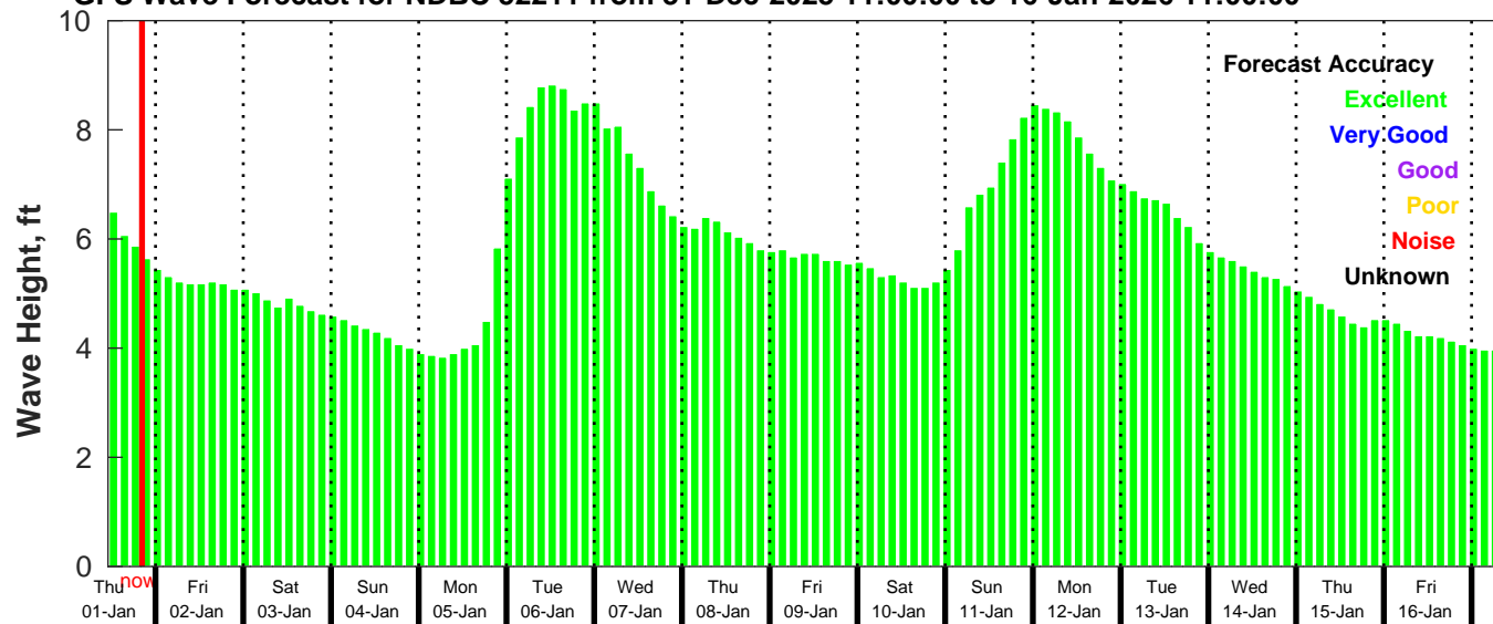
GFS Wave Forecast for NDBC 52211 from 31-Dec-2025 11:00:00 to 16-Jan-2026 11:00:00
