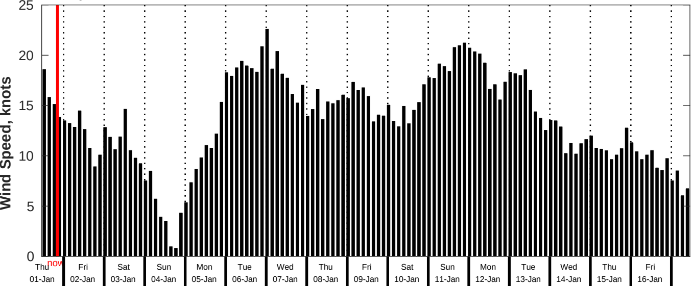
GFS Wind Speed Forecast for NDBC 52211 from 31-Dec-2025 11:00:00 to 16-Jan-2026 11:00:00
