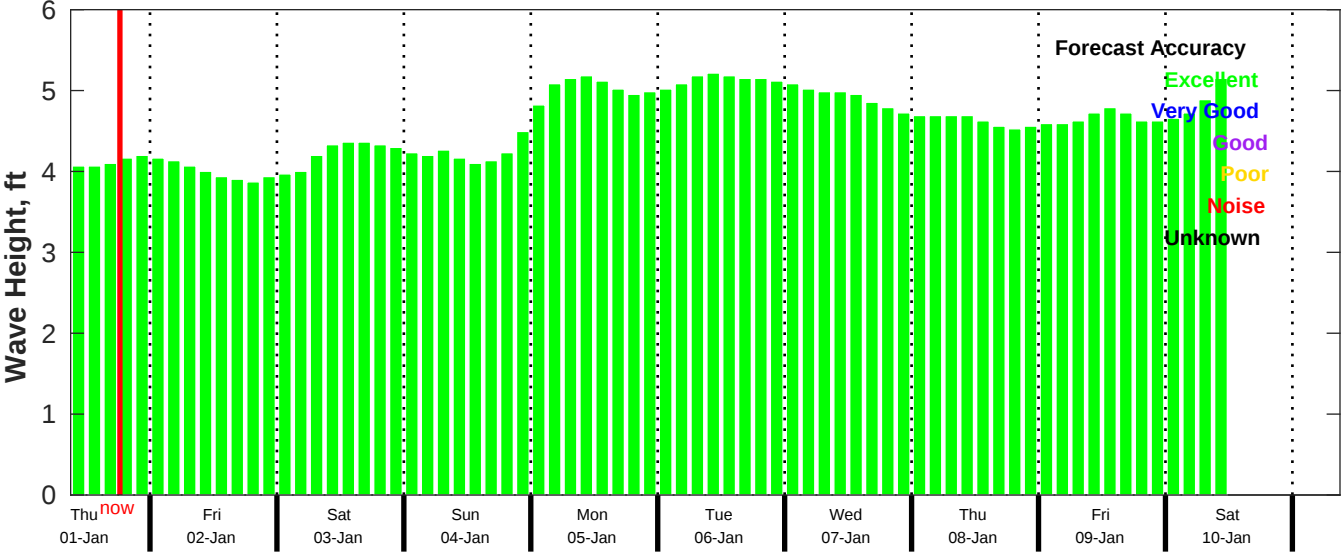
CMEMS Wave Forecast for NDBC 52212 from 31-Dec-2025 09:00:00 to 10-Jan-2026 09:00:00
