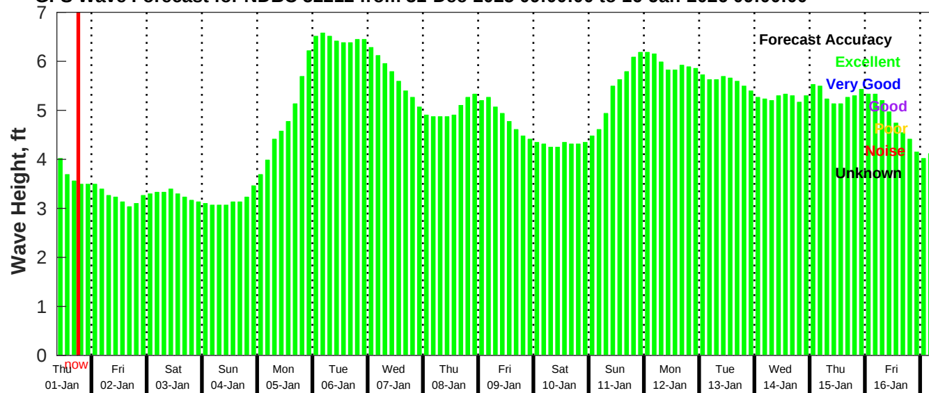
GFS Wave Forecast for NDBC 52212 from 31-Dec-2025 09:00:00 to 16-Jan-2026 09:00:00
