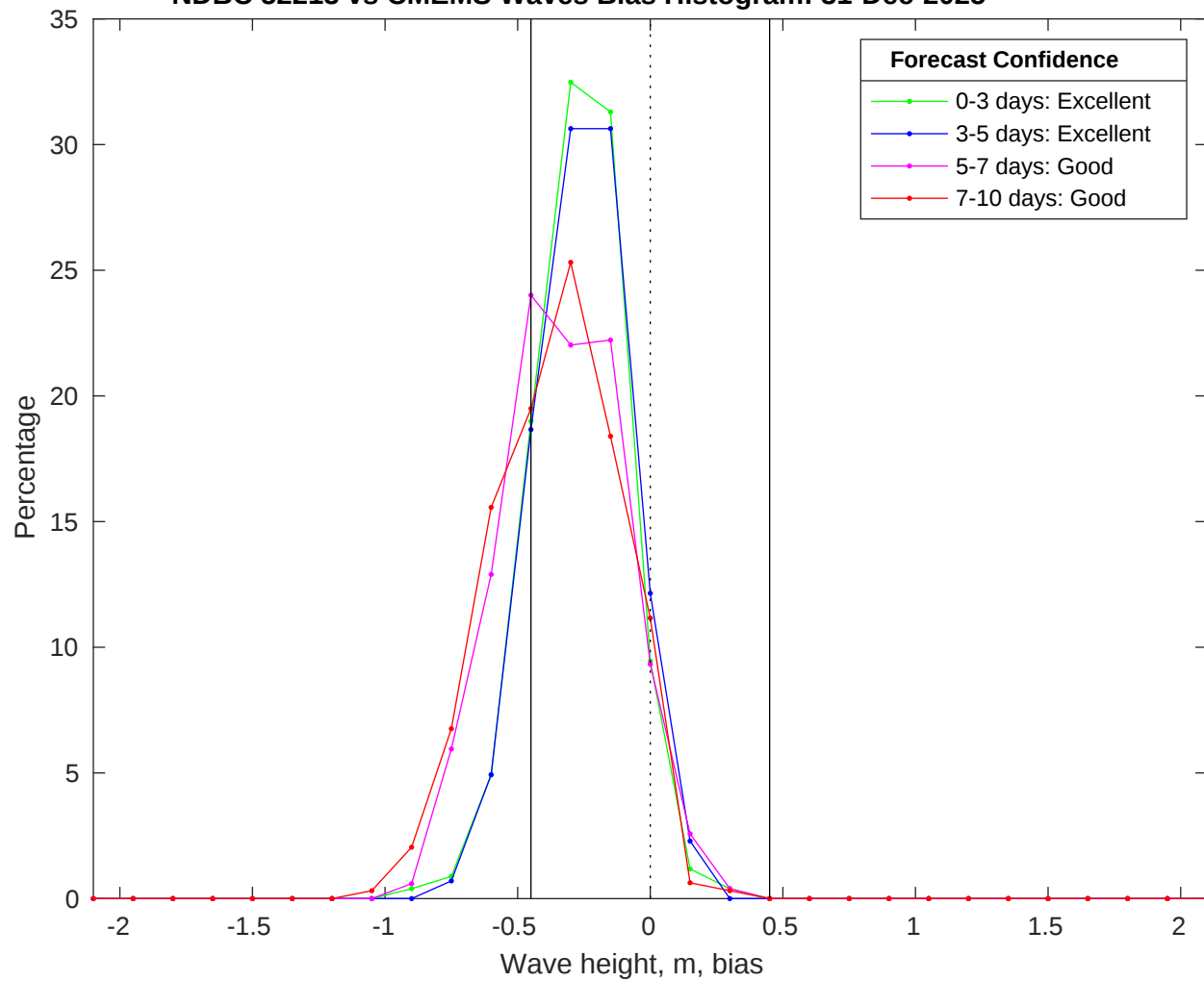
NDBC 52213 vs CMEMS Waves Bias Histogram: 31-Dec-2025
