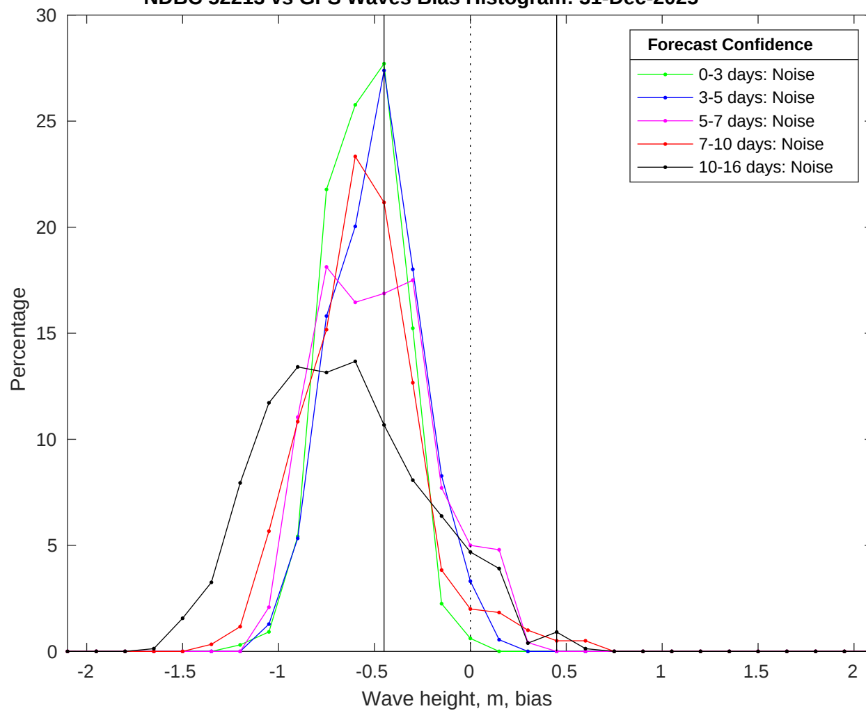
NDBC 52213 vs GFS Waves Bias Histogram: 31-Dec-2025
