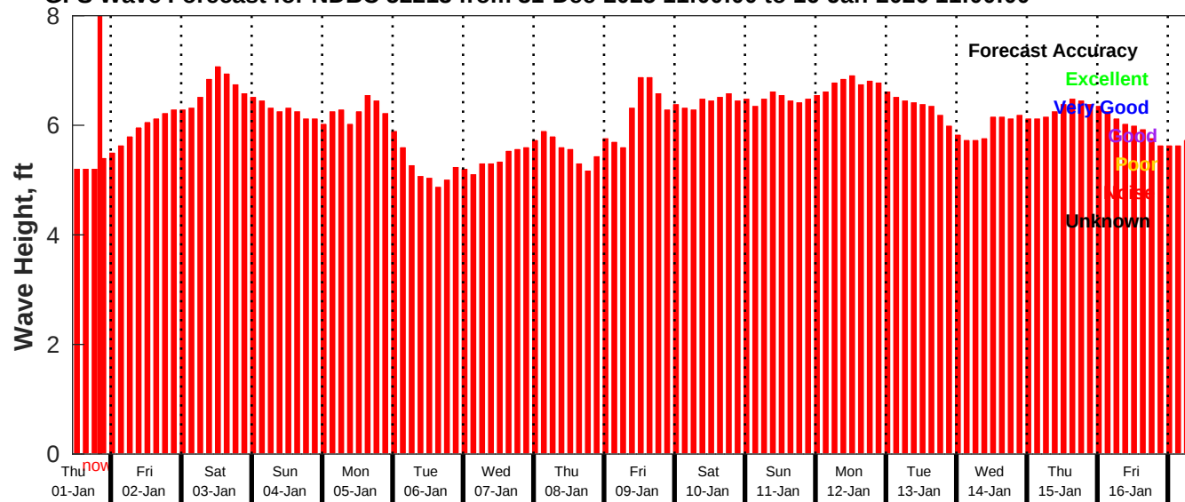
GFS Wave Forecast for NDBC 52213 from 31-Dec-2025 11:00:00 to 16-Jan-2026 11:00:00
