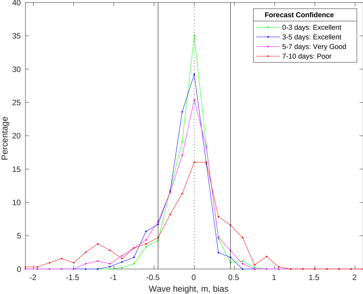
NDBC 41004 vs CMEMS Waves Bias Histogram: 01-Jan-2026
