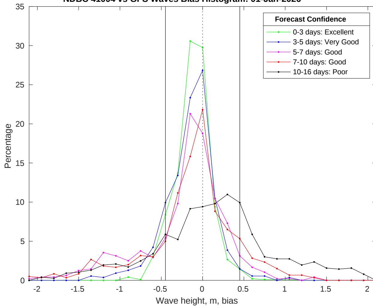
NDBC 41004 vs GFS Waves Bias Histogram: 01-Jan-2026
