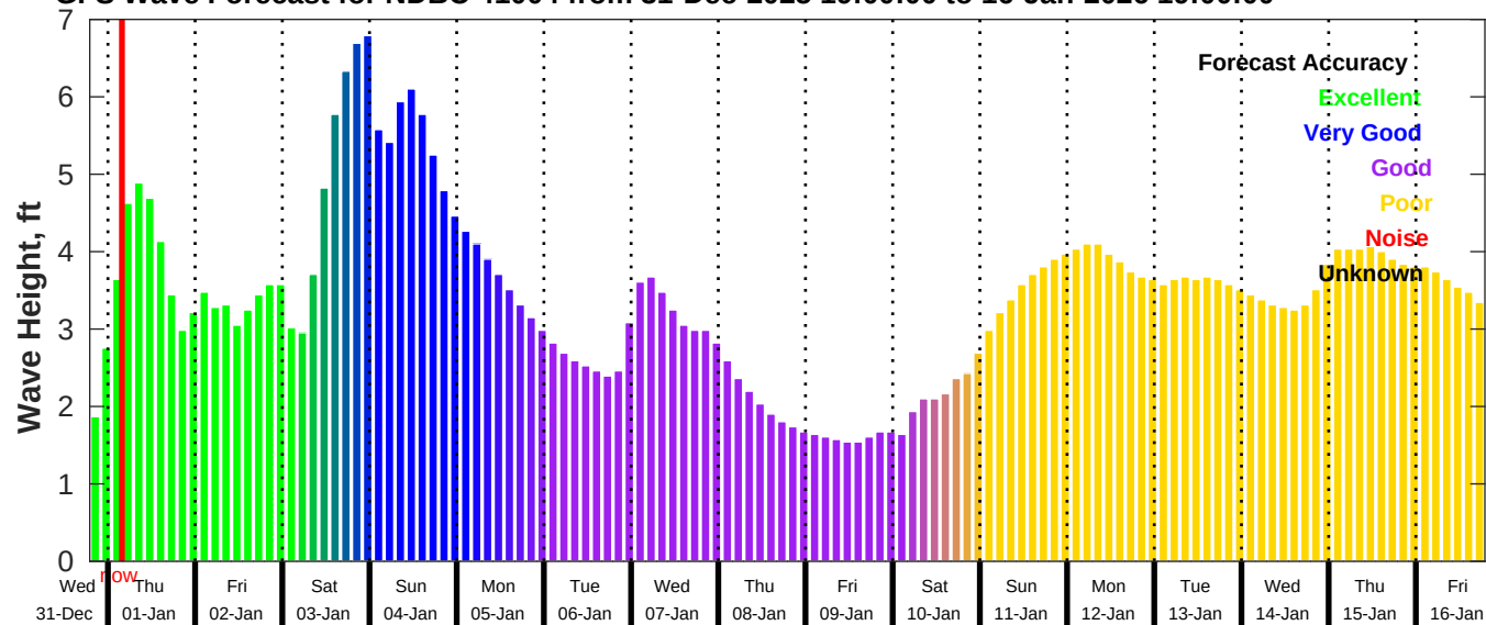
GFS Wave Forecast for NDBC 41004 from 31-Dec-2025 19:00:00 to 16-Jan-2026 19:00:00
