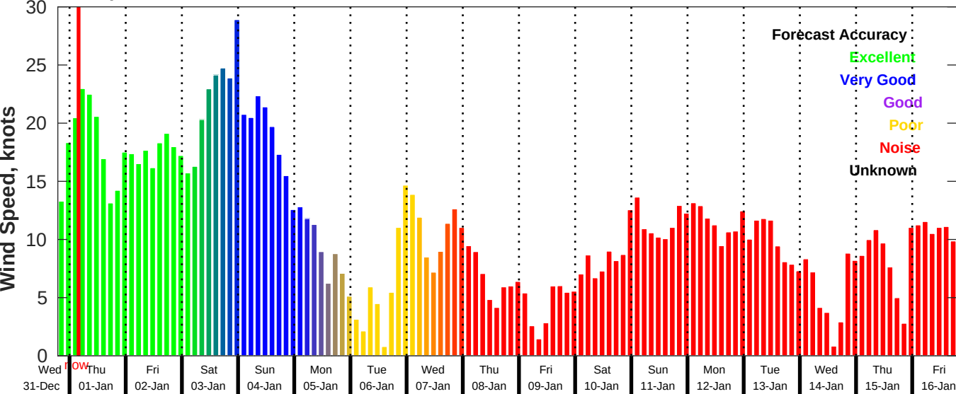
GFS Wind Speed Forecast for NDBC 41004 from 31-Dec-2025 19:00:00 to 16-Jan-2026 19:00:00
