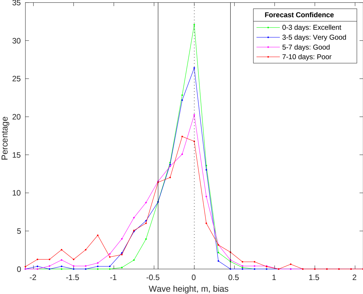
NDBC 41013 vs CMEMS Waves Bias Histogram: 01-Jan-2026
