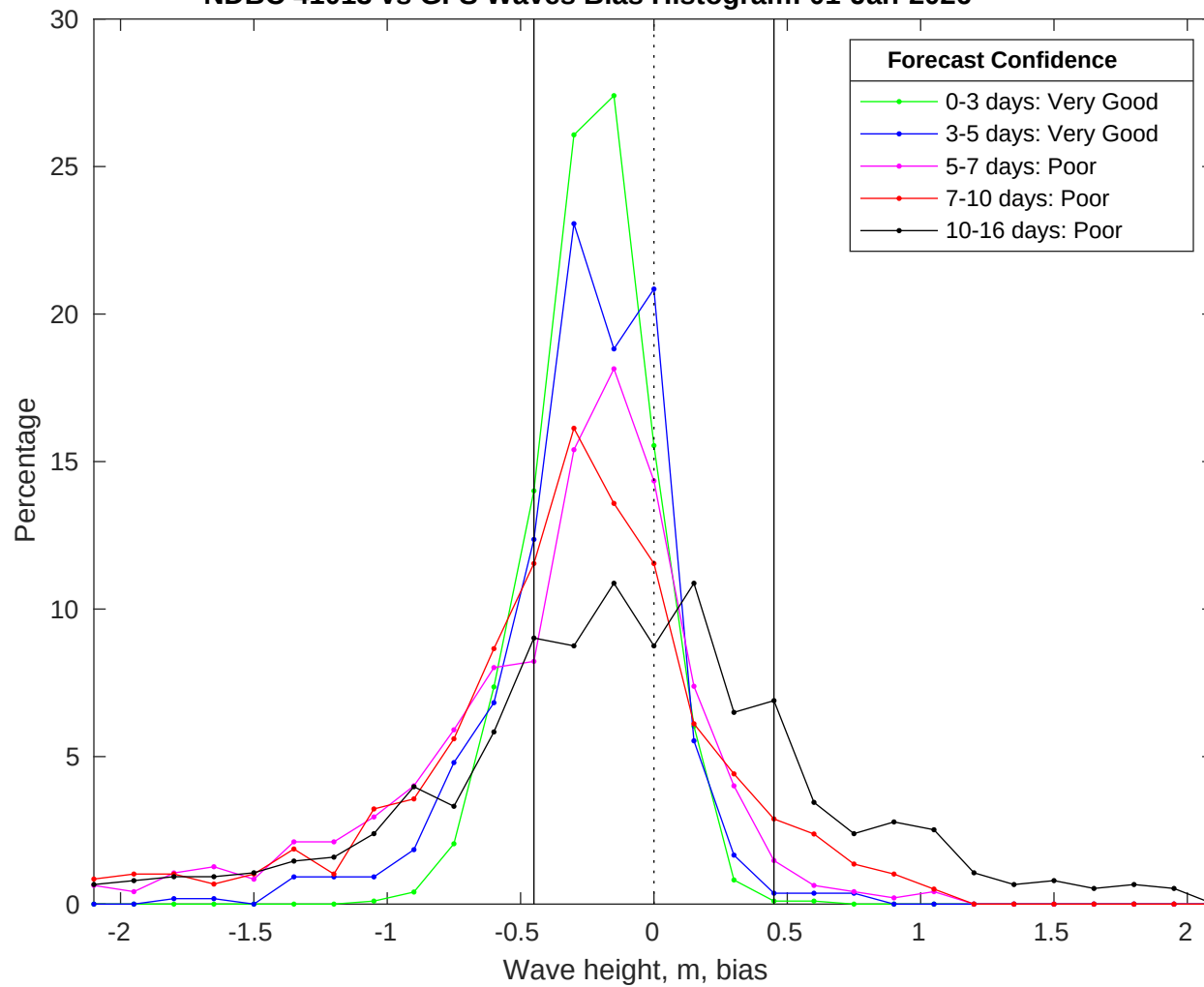
NDBC 41013 vs GFS Waves Bias Histogram: 01-Jan-2026
