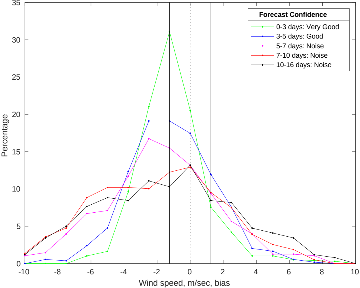
NDBC 41013 vs GFS Winds Bias Histogram: 01-Jan-2026
