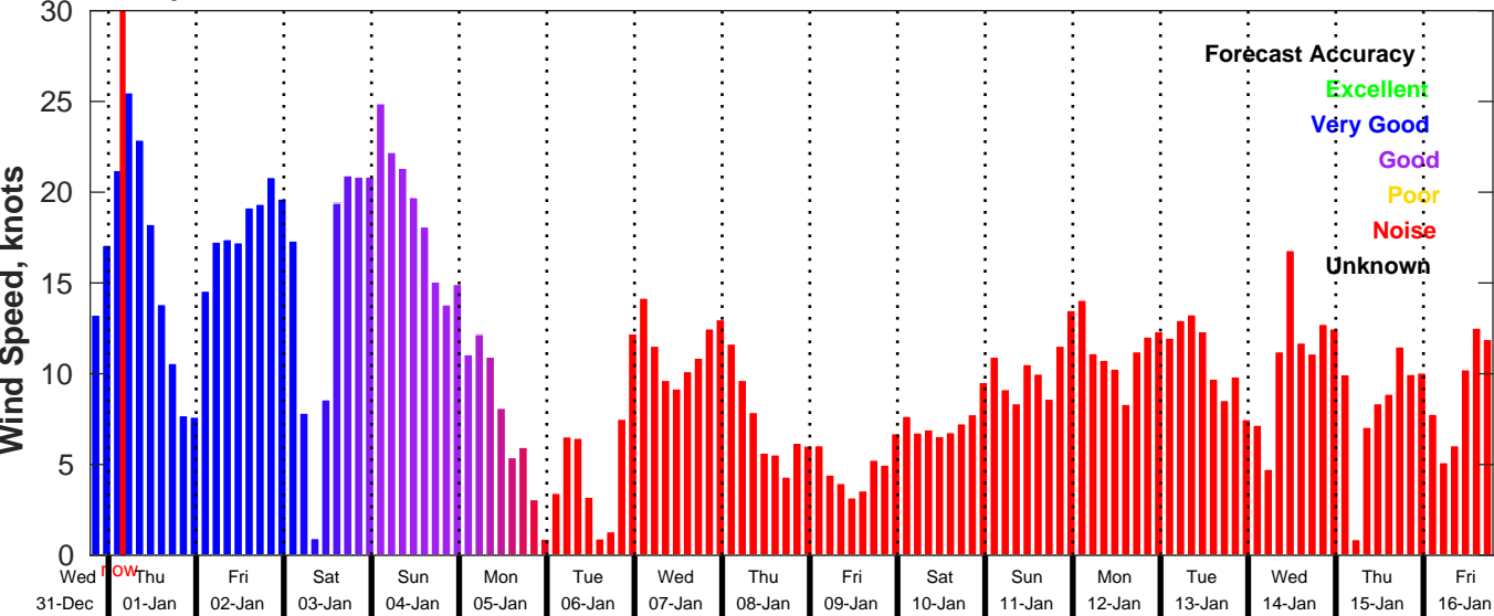
GFS Wind Speed Forecast for NDBC 41013 from 31-Dec-2025 19:00:00 to 16-Jan-2026 19:00:00
