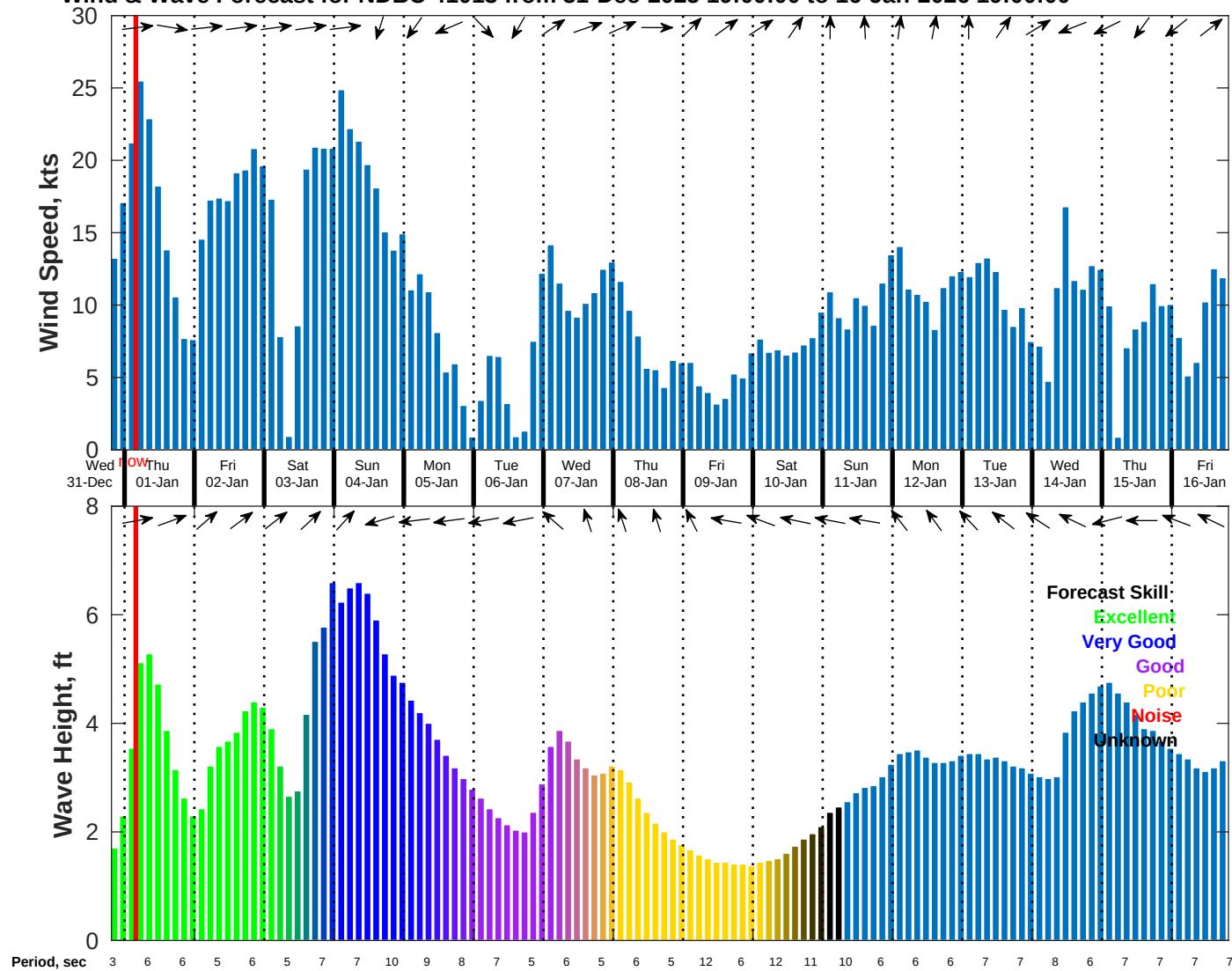
Wind & Wave Forecast for NDBC 41013 from 31-Dec-2025 19:00:00 to 16-Jan-2026 19:00:00
