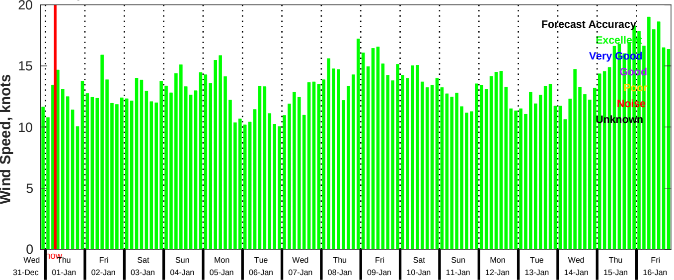
GFS Wind Speed Forecast for NDBC 41040 from 31-Dec-2025 21:00:00 to 16-Jan-2026 21:00:00
