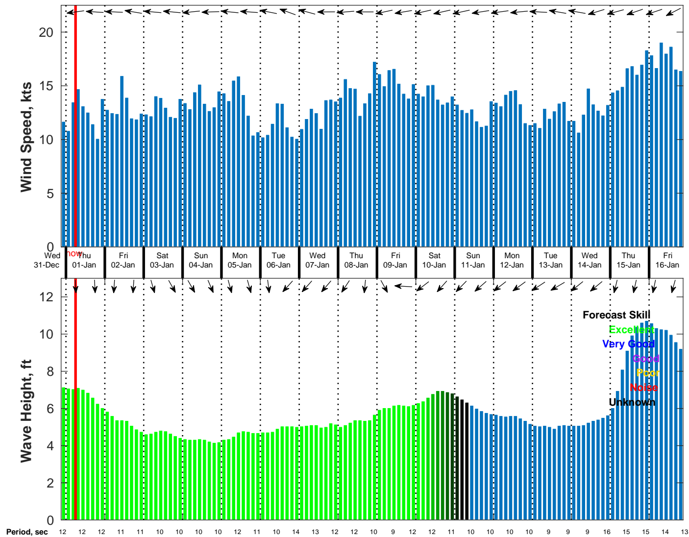
Wind & Wave Forecast for NDBC 41040 from 31-Dec-2025 21:00:00 to 16-Jan-2026 21:00:00
