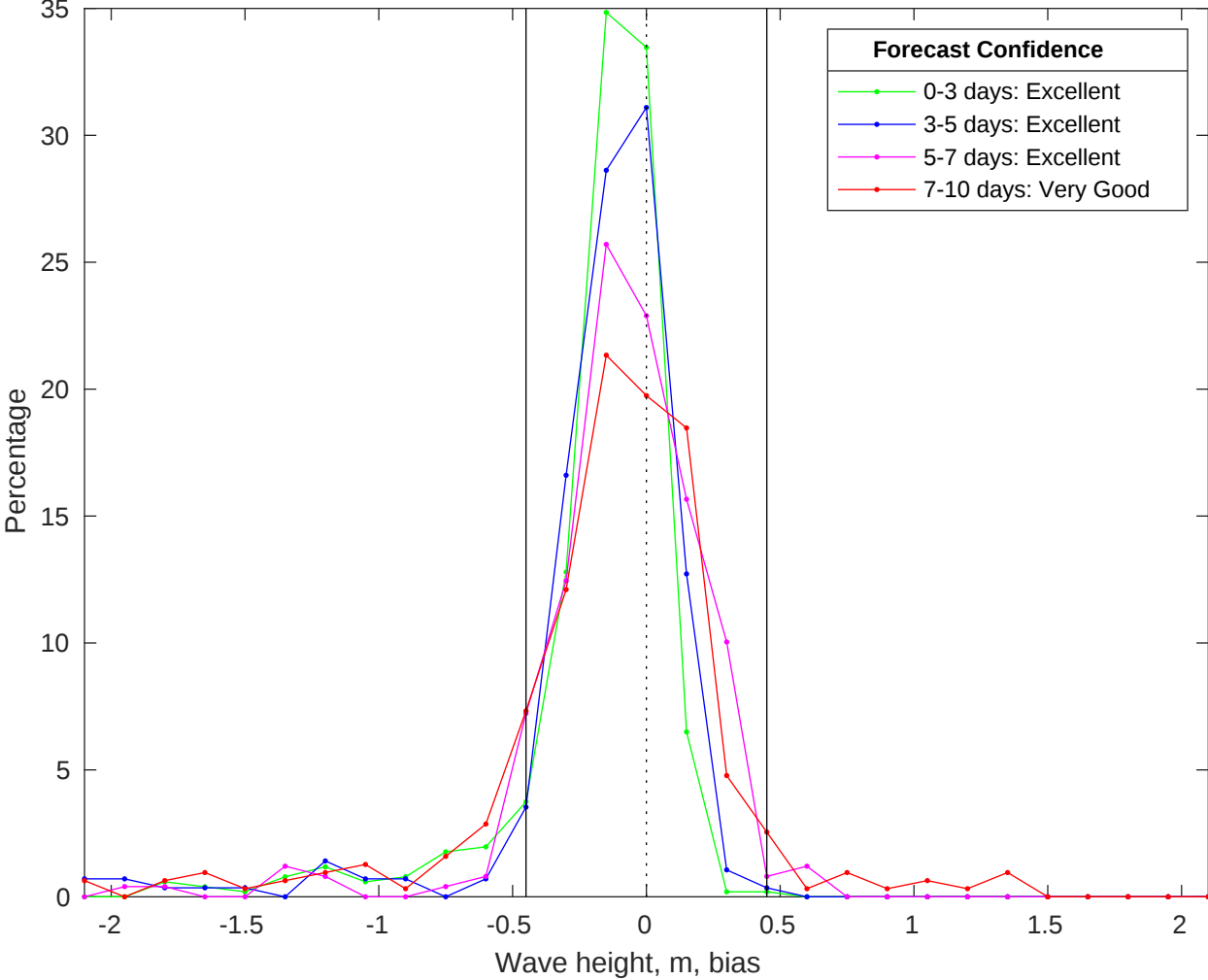
NDBC 42019 vs CMEMS Waves Bias Histogram: 01-Jan-2026
